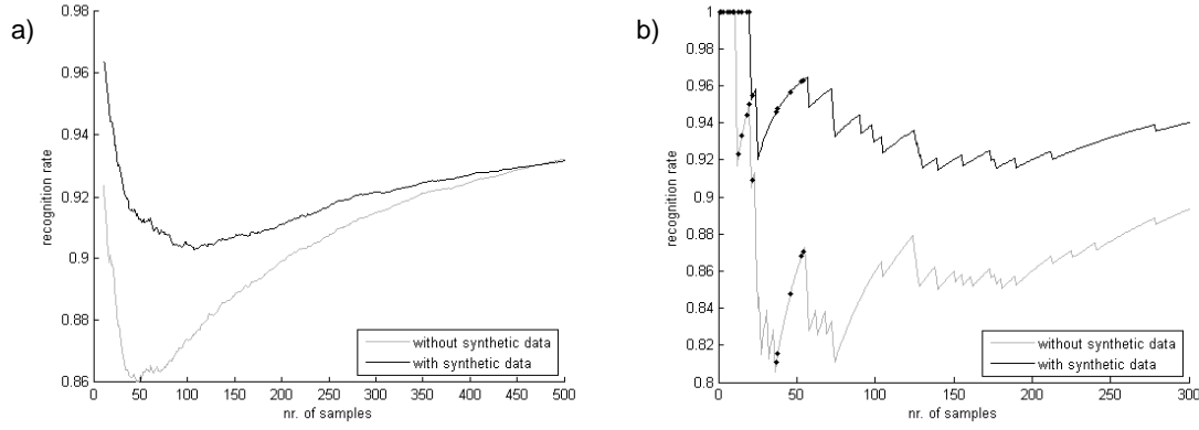
Figure 2. Comparison of recognition rate when using only original data to the use of synthetic data, without (a) and with (b) highlighted times of addition of new class (dots).
