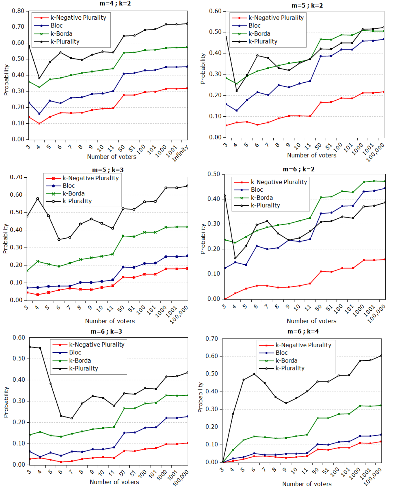
Figure 1: The probability of type 1 for the agreement between Chamberlin-Courant and other multiwinner scoring rules
