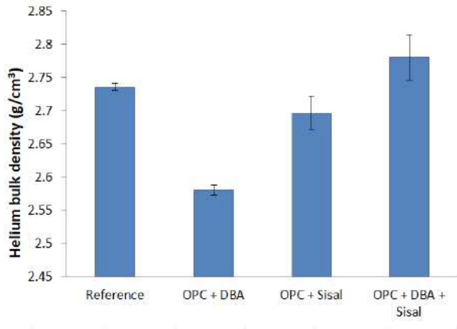
Fig. 9: Helium bulk density (mean values and standard deviations) of the different composite mixtures
