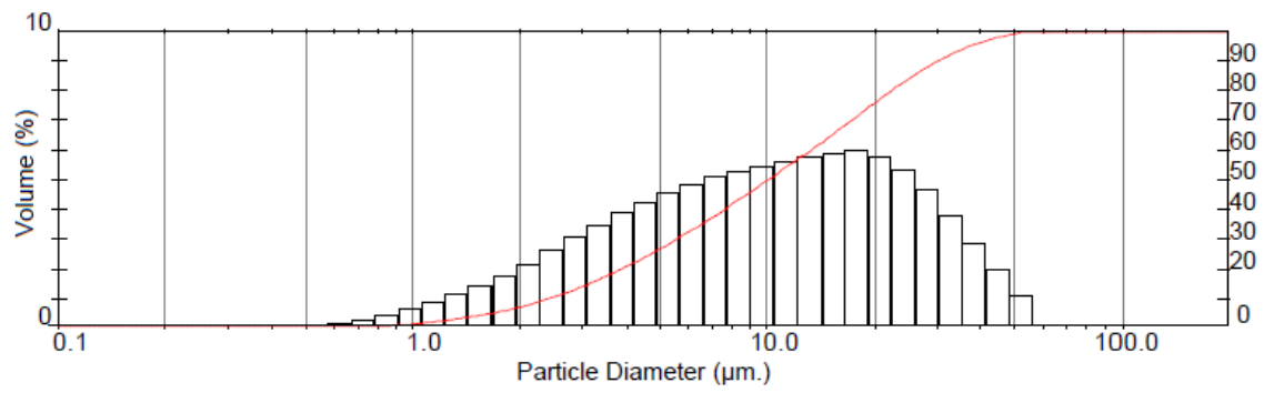
Fig. 6: Particle size distribution of the ordinary Portland cement (OPC)
