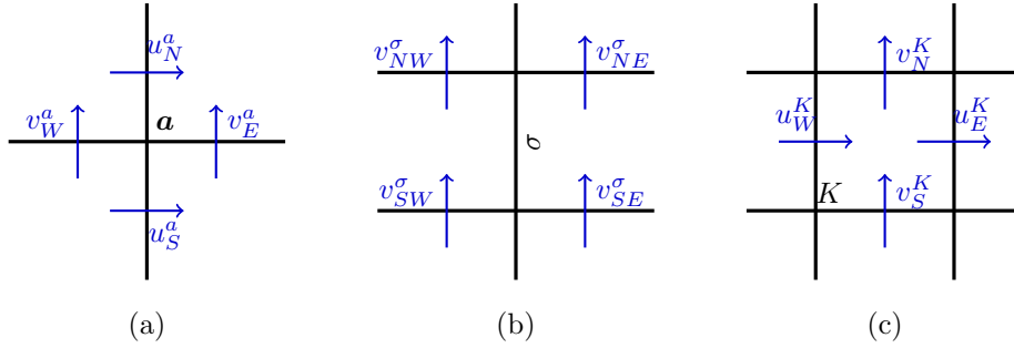
FIGURE 7. Local notations for the proof of the discrete Korn lemma.
