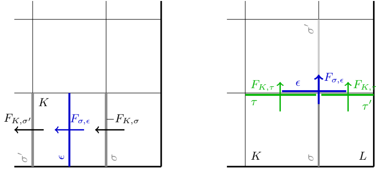
FIGURE 4. In the two-dimensional case, primal mass fluxes involved in the computation of the dual mass flux associated to \epsilon = \sigma|\sigma' \in \tilde{\mathcal{E}}_{\text{int}}^{(1)} . Left: for \epsilon \perp e^{(1)} . Right: for \epsilon \perp e^{(2)} .
