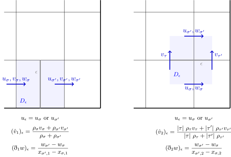
FIGURE 5. Velocities and velocity partial derivative over D_\epsilon involved in the right-hand side of Equation (28), in the two-dimensional case, for i = 1 . Left: j = 1 . Right: j = 2 .
