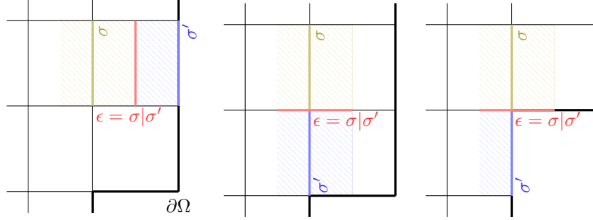
FIGURE 2. Definition of \epsilon = \sigma|\sigma' in the two-dimensional case for (\sigma, \sigma') \in \mathcal{E}^{(1)} . Left: \epsilon \in \tilde{\mathcal{E}}^{(1,1)} . Middle: \epsilon \in \tilde{\mathcal{E}}^{(1,2)} \cap \tilde{\mathcal{E}}_{\text{int}}^{(1)} . Right: \epsilon \in \tilde{\mathcal{E}}^{(1,2)} \cap \tilde{\mathcal{E}}_{\text{rec}}^{(1)} .
