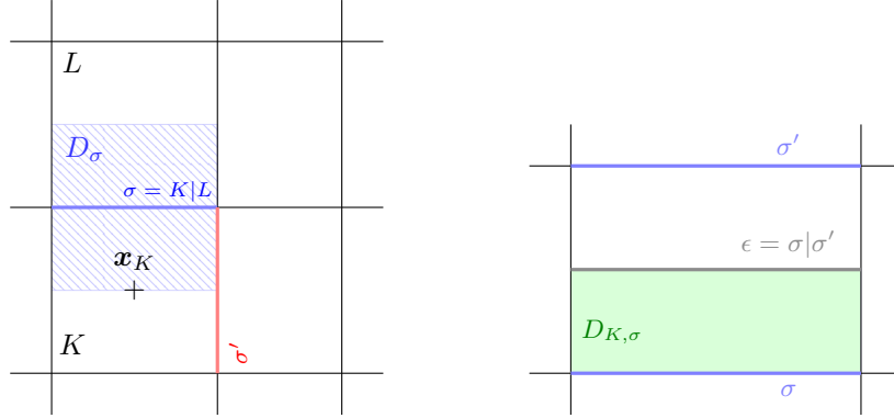
FIGURE 1. Representation of (\mathcal{M}, \mathcal{E}) for d = 2 .
