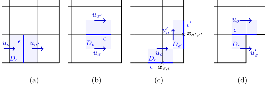
FIGURE 3. (i, j) - gradient cells in the two-dimensional case.
