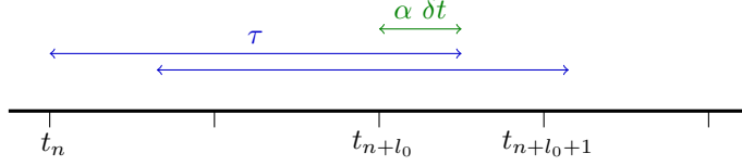
FIGURE 6. Notations for the velocity time translates estimates.
